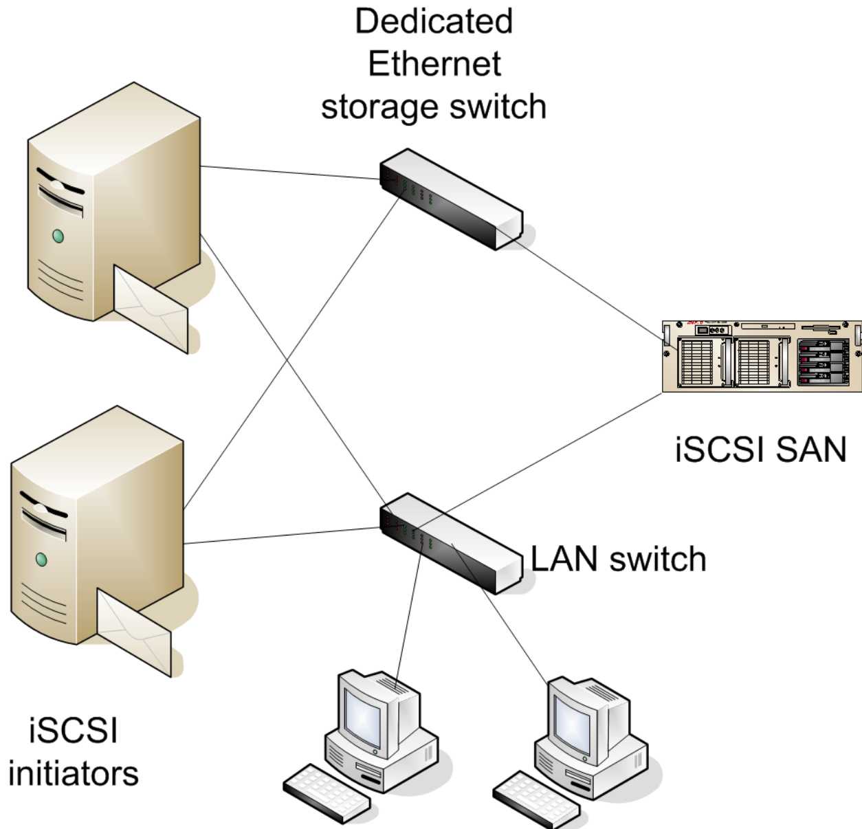
Figure 3.3: Providing a dedicated network for iSCSI storage.
